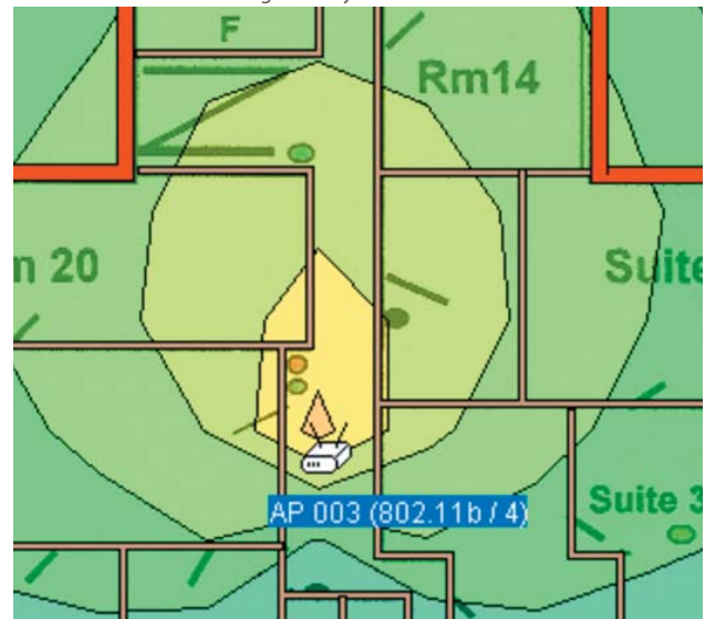
Floor Plan - with wifi coverage overlay
